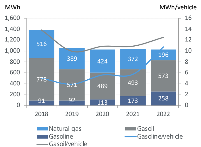
Evolution of fuel consumption
